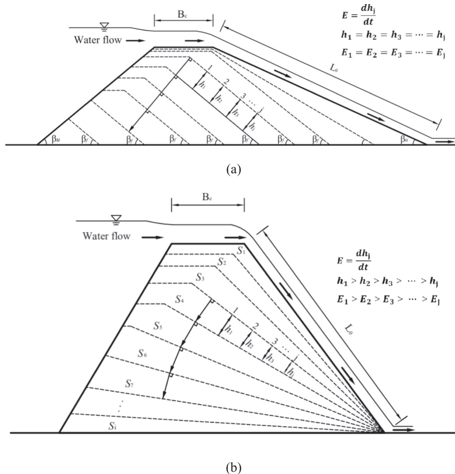
Fig. 1. (a) Evolution of longitudinal breach profile of the landslide dam due to overtopping failure by Chang and Zhang (2010) (Modified); (b) evolution of longitudinal breach profile of the landslide dam due to overtopping failure by Zhong et al. (2018) (Modified). B_c means the width of dam crest and L_0 is the length of downstream slope.
