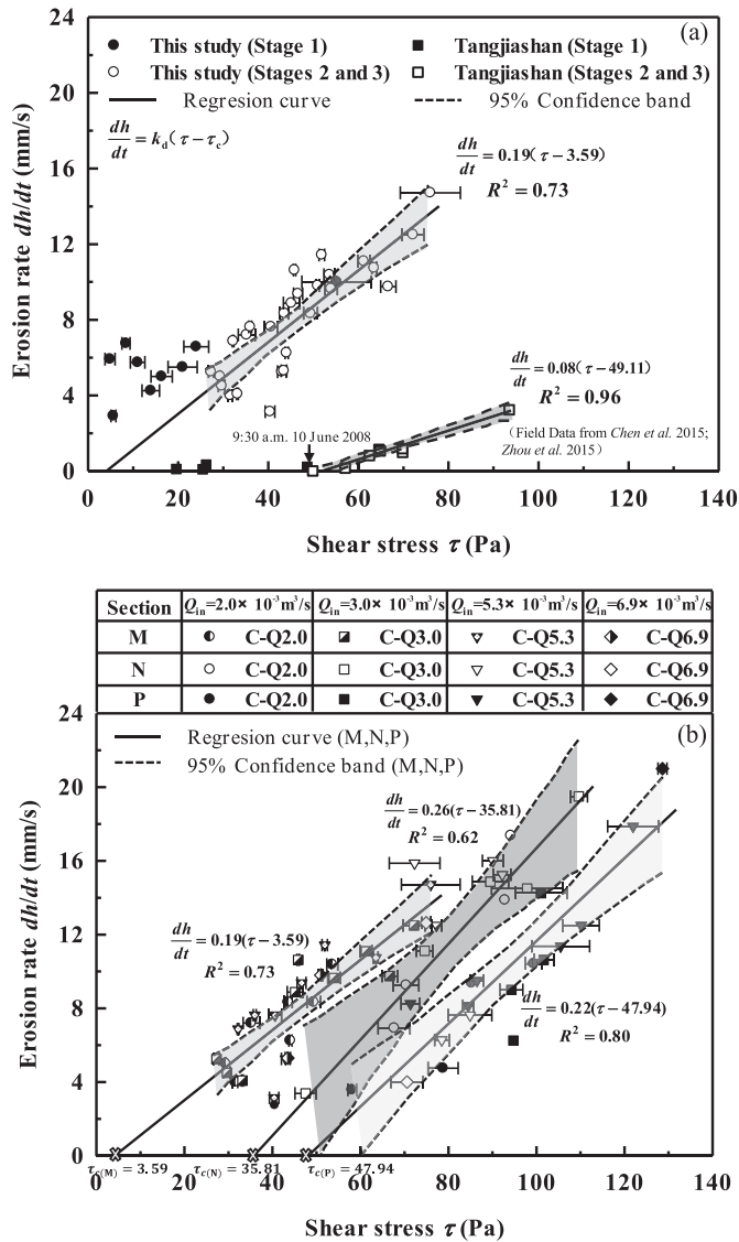
Fig. 14. (a) A representative (Section M) relationship between erosion rate and shear stress obtained from the experiments and from the Tangjiashan landslide dam (cf. Chen et al., 2015; G.G.D. Zhou et al., 2015; X.Q. Zhou et al., 2015). (b) The relationship between erosion rate and shear stress at different sections (M, N, P) for all experiment set-up during Stages 2 and 3. Error bars for shear stress express standard deviations of distributed measurements, and linear line, R^2 values summarize results of regression analysis. The shadows are based on a 95% confidence interval.
