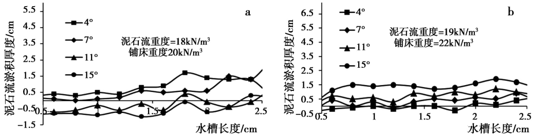
( a. \gamma_c = 18 \text{ kN/m}^3 \gamma_b = 20 \text{ kN/m}^3 ; b. \gamma_c = 19 \text{ kN/m}^3 \gamma_b = 22 \text{ kN/m}^3 )
