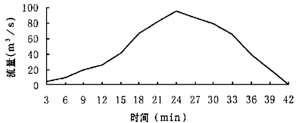
图 5 1994-06-16 大凹子沟泥石流流量过程曲线图 Fig. 5 The debris flow discharge process in Dawazi gully on June 16, 1994
